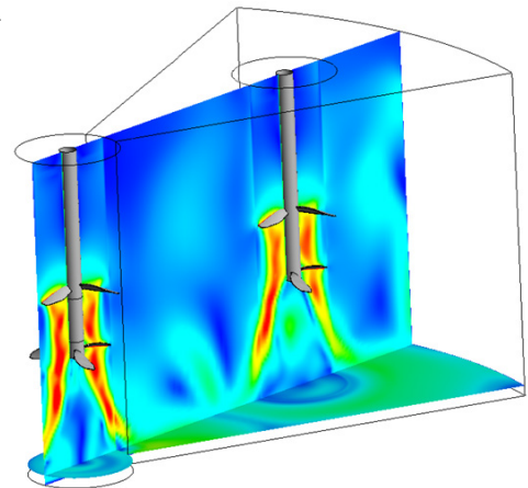
CFD simulation of an attack tank in phosphoric acid production.
